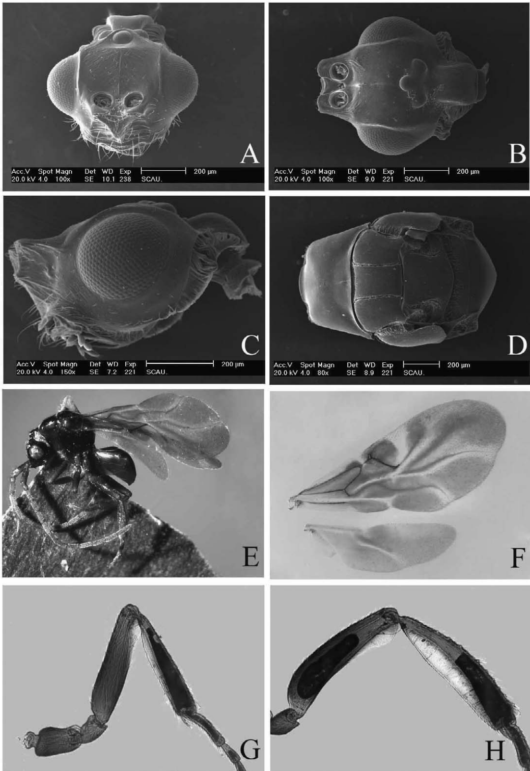
Fig. 4. Loboscelidia striolata sp. nov. A-C. Head of paratype (A. frontal view; B. dorsal view; C. lateral view). D. Meosoma, dorsal view. E. Habitus, lateral view. F. Wings. G. Middle leg. H. Hind leg.
