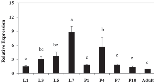
Fig. 3. Expression patterns of the BdEcR-B1 in different developmental stages of B. dorsalis (bar graph represented Mean ± SE; different letters above each bar indicated the significant difference, P < 0.05 , LSD in ANOVA). L and P represent larval and pupa, respectively.
