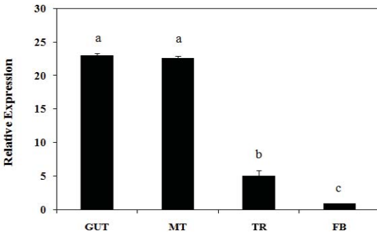
Fig. 4. Expression patterns of the BdEcR-B1 in different tissues of larval B. dorsalis (bar graph represented Mean ± SE; different letters above each bar indicate significant difference, P < 0.05 , LSD in ANOVA). FB, GUT, MT, and TR represent fat body, gut, Malpighian tubule, and trachea, respectively.
