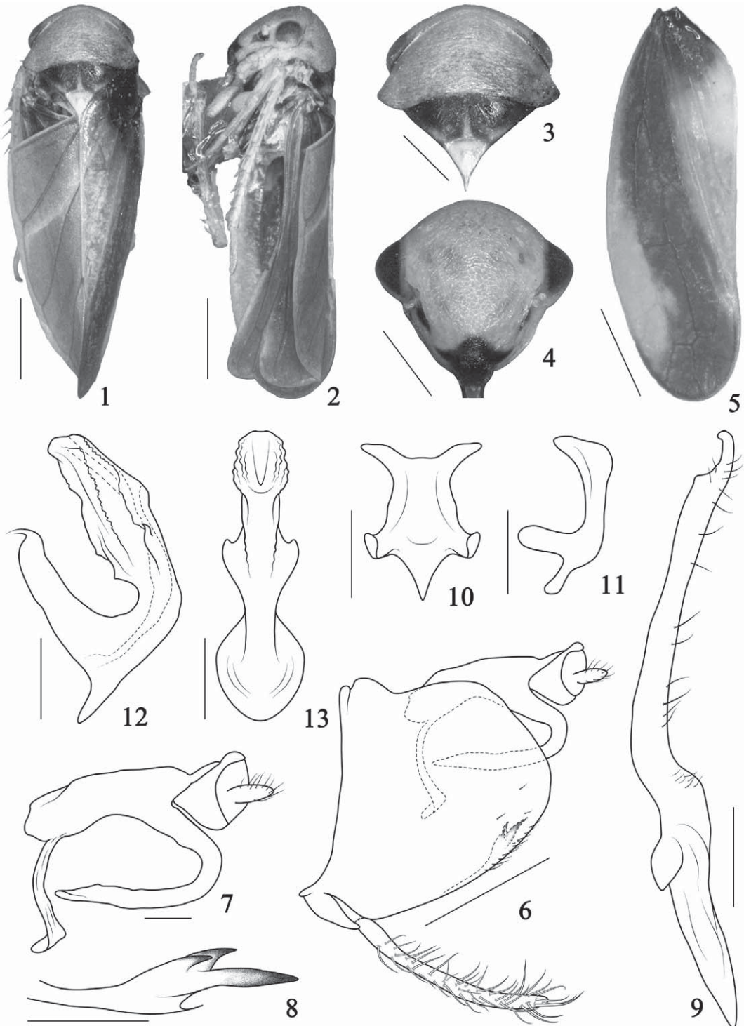
Figs. 1-13. Pedioipsoides (Celopsis) rhombica Li, Dai & Li sp. nov. 1. Habitus, dorsal view; 2. Habitus, lateral view; 3. Cephalothorax, dorsal view; 4. Face; 5. Fore wing; 6. Pygofer, subgenital plate and segment X, lateral view; 7. Anal tube and dorsal connective, lateral view; 8. Pygofer ventral process, inner lateral view; 9. Style, dorsal view; 10. Connective, dorsal view; 11. Connective, lateral view; 12. Aedeagus, lateral view; 13. Aedeagus, ventral view. Scale bars for 1-2, 5 = 1.0 mm, for 3-4, 6 = 0.5 mm, for 7-13 = 0.2 mm. Note : This plate is show in color in Suppl. Figs. 1-13 online in Florida Entomologist 96(3) (2013) at http://purl.fcla.edu/fcla/entomologist/browse .
