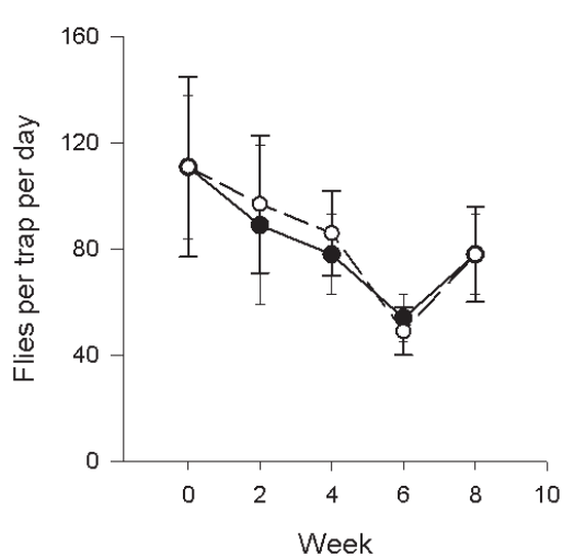
Fig. 1. Numbers of Bactrocera dorsalis male flies captured in traps baited with methyl eugenol (ME) alone or a mixture of ME and raspberry ketone (RK, a natural analogue of cue lure). Comparisons involved 3 mixtures in ME:RK ratios (wt:wt) of 95:5, 90:10, and 85:15. Symbols represent means ( \pm SE) of 15 traps per lure type at 2 wk intervals over an 8 wk sampling period.
