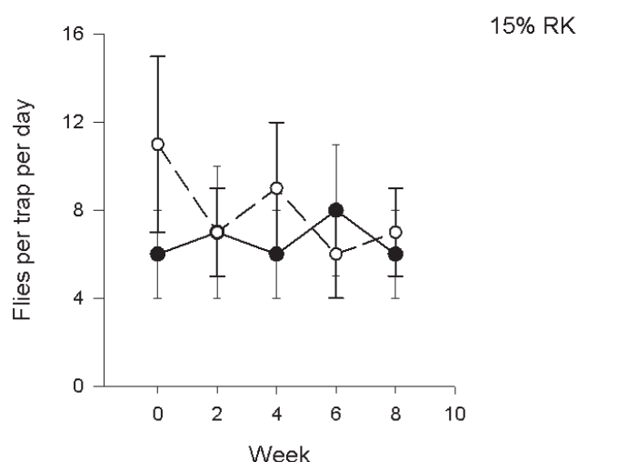
Fig. 2. Numbers of Bactrocera cucurbitae male flies captured in traps baited with cue lure (CL) alone or a mixture of methyl eugenol (ME) and raspberry ketone (RK, a natural analogue of cue lure). Comparisons involved 3 mixtures in ME:RK ratios (wt:wt) of 95:5, 90:10, and 85:15. Symbols represent means ( \pm SE) of 15 traps per lure type at 2 wk intervals over an 8 wk sampling period.
