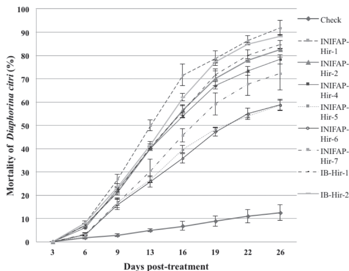
Fig. 1. Overall mean mortality of Diaphorina citri adults caused by conidia of 8 Hirsutella citriformis strains applied by contact (3 separate bioassays) under controlled conditions ( 26 \pm 1 °C, 76 \pm 4\% RH, 16:8 h L:D photoperiod). Error bars represent the standard error ( n = 7 ).
