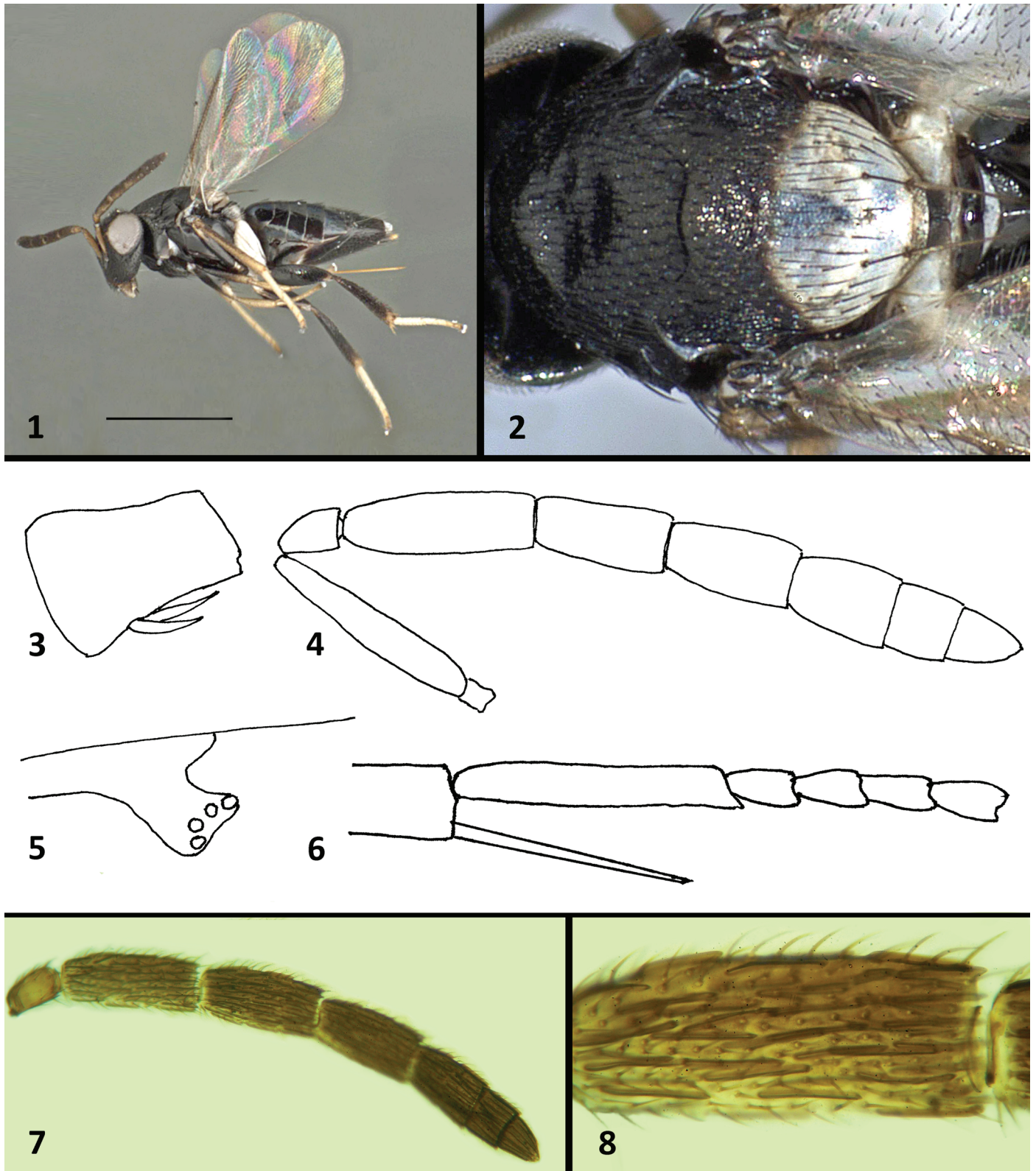
Figs. 1–8. Coccophagus funiculatus , sp. nov., female. 1, Lateral view of body; 2, mesoscutum, dorsal view; 3, mandible; 4, antenna; 5, stigmal and postmarginal veins; 6, mid-tarsus and mid-tibial spur; 7, antenna with sensilla; 8, 1st funicular segment.
