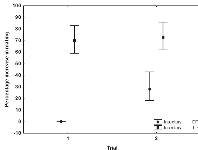
Fig. 3. The mean percentage increase in mating of Cactoblastis cactorum females in mating cage bioassays as influenced by the insectary (DPI or TIF) and the trial conducted before (trial 1) and after (trial 2) quality improvements were made to the rearing and handling protocols at the DPI insectary. Vertical bars denote 0.95 confidence intervals.
