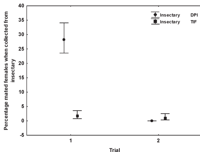
Fig. 2. The mean percentage of Cactoblastis cactorum females that were mated at time of collection from the insectaries (DPI or TIF) and the trial conducted before (trial 1) and after (trial 2) quality improvements were made to the rearing and handling protocols at the DPI insectary. Vertical bars denote 0.95 confidence intervals.
