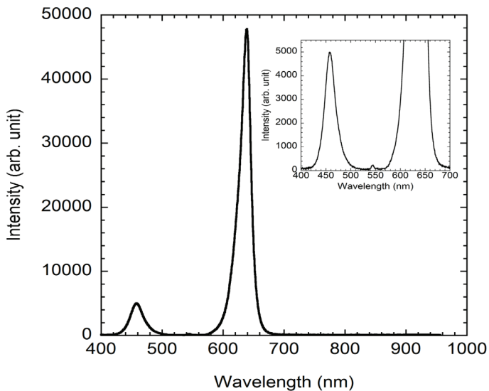
Fig. 1. Light emission spectrum of the W2238 LED grow panel over the visible spectrum and into the near infrared. The inset spectrum is zoomed vertically to show details of any weaker emissions.
