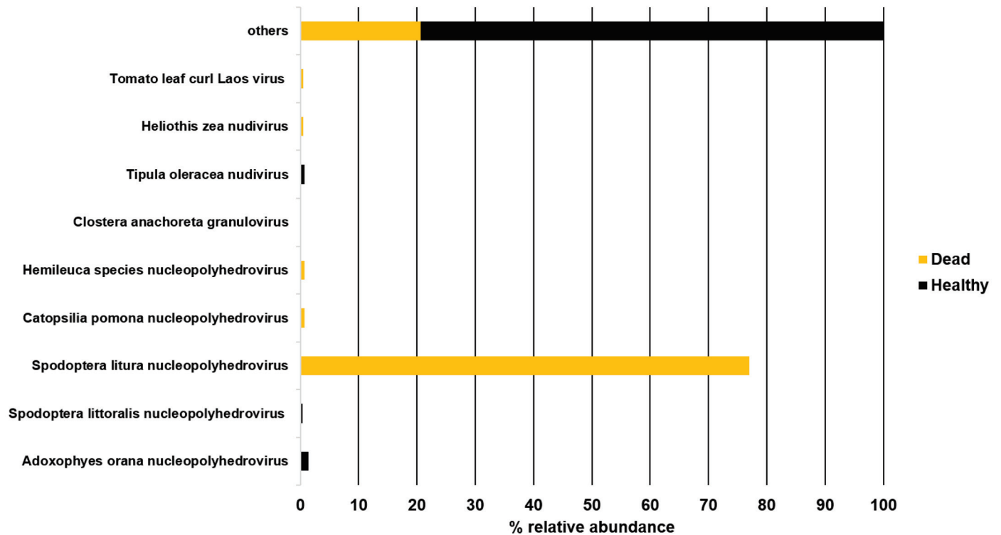
Fig. 2. Relative abundance of diversity of viruses found in the metagenomic analysis of dead and healthy larvae of Spodoptera frugiperda .
