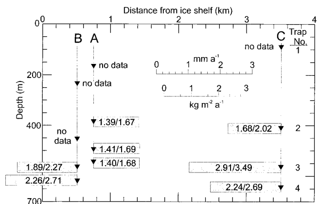
FIGURE 2. Location of the sediment traps (triangles) with respect to water depth and distance from Müller Ice Shelf front in March 1998. In each case, the sea floor was 5 m below the lowest trap. Traps are numbered from the top down as shown on the right. Bars show the accumulation of sediment in \text{mm a}^{-1} based on the volume of sediment in each trap at the time of recovery and \text{kg m}^{-2} \text{ a}^{-1} based on a mean bulk density of 1200 \text{ kg m}^{-3} .
