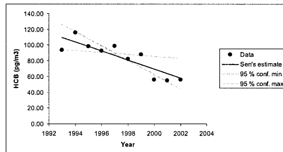
FIGURE 6. Time trend for OCs in air+aerosol at Zeppelin. In addition to data points (black dots) the figure also shows Sens trend estimate (line) and the lines for \pm 95\% confidence interval (broken lines).
