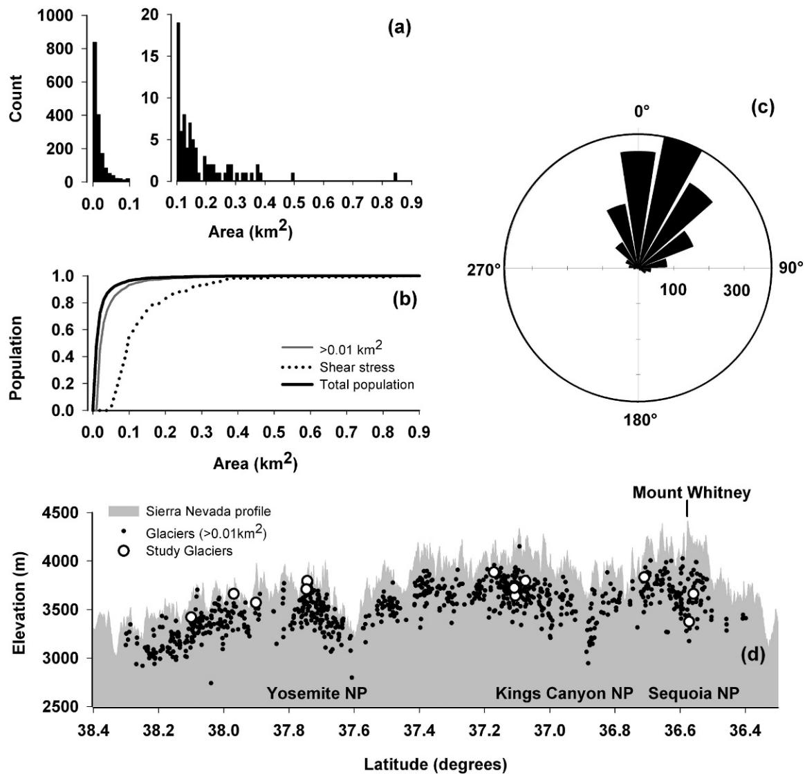
FIGURE 2. Characteristics of the population of glaciers and perennial snowfields in the Sierra Nevada, California: (a) population as a function of area (km 2 ), note change in y-axis for glaciers >0.01 km 2 ; (b) cumulative sum with area for the total population, for glaciers >0.01 km 2 , and for the population of features with an estimated basal shear stress >10 5 Pa; (c) total population as a function of aspect, using 20° bins; and (d) the north-to-south distribution of the glacier population >0.01 km 2 (black dots) and study glaciers (white circles) overlaid on elevation of the Sierra Nevada (gray).
