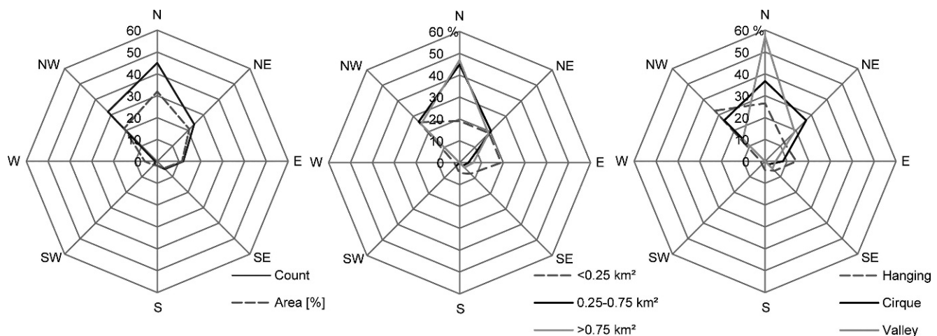
FIGURE 9. Number of glaciers and glaciated area (%) in relation to their main aspect (left), percentage distribution relating to glacier size classes (middle), and percentage distribution relating to categories of glaciers (right).
