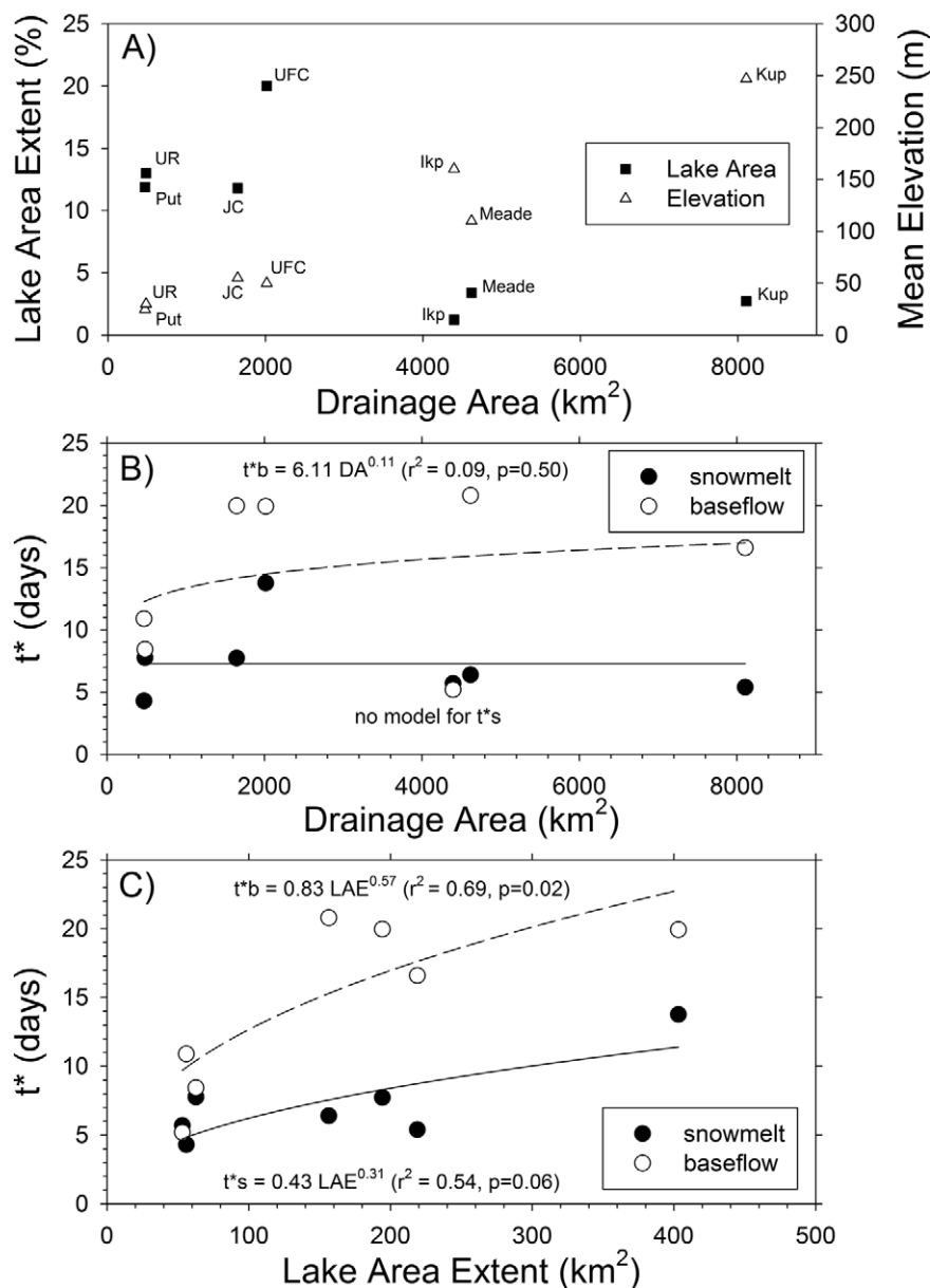
FIGURE 9. Comparison among major Alaskan Arctic Coastal Plain watersheds according to lake area, elevation, and size (A), recession coefficients ( t^* ) and drainage area (B), and recession coefficients ( t^* ) and lake area extent (C) (UFC = Upper Fish Creek, JC = Judy Creek, UR = Ublutuooh River, Meade = Meade River, Ikp = Ikpikpuk River, Kup = Kuparuk River, and Put = Putuligayuk River).
