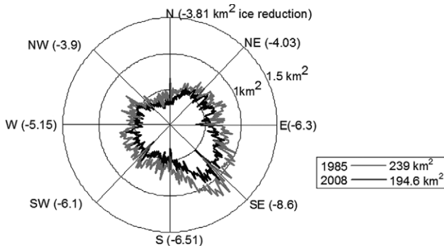
FIGURE 6. Orientation of the glaciated area in the San Lorenzo region in 1985 (gray) and 2008 (black). Values in parentheses indicate absolute ice losses in square kilometers for each cardinal sector. Note that although most glaciers are located on slopes oriented towards the southeast, the percentage reduction in glaciated area is roughly similar for all cardinal sectors (ranging between 14% and 23%).
