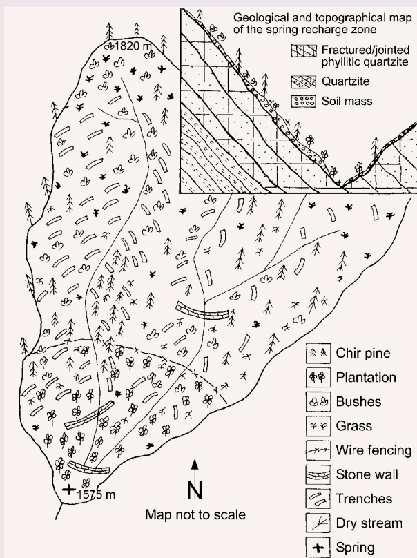
FIGURE 2 Bioengineering treatments in the recharge zone of a spring in Dugar Gad Watershed. (Sketch by authors)
