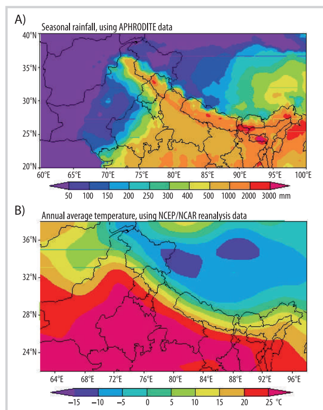
FIGURE 3 (A) Seasonal (June–September) rainfall (mm) based on APHRDITE data; (B) annual average temperature (°C) based on NCEP/NCAR reanalysis data for 1961–1990.
