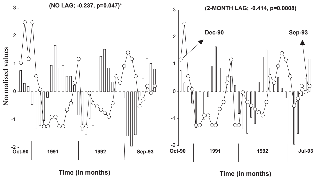
Fig. 2. Immediate and lag effects of maximum temperature (a) and minimum temperature (b) on the population of D. pinguis at Tamparam. Abiotic factors are represented as bars and population as lines. Values are normalized. Correlation coefficient values with significance levels are given within parentheses. * refers to p level as insignificant after subjection to a sequential Bonferroni test. The 'month-year' indicated on the x-axis refers to the beginning and end of abiotic factor data, with vertical lines marking the beginning of each year. The 'month-year' indicated beside the arrow pointer refers to the beginning and end of the population data with lag and with respect to the corresponding abiotic factor.
