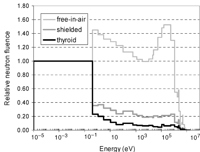
FIG. 2. Neutron fluence spectra for survivor E90 (DS02 ground range: 893 m) as provided by DS02. Light gray line: free-in-air 1 m above ground; dark gray line: including surrounding structures; black line: within thyroid.
