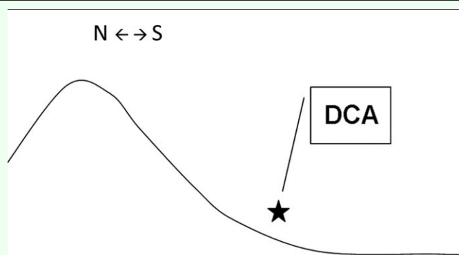
Figure 4. Diagram of a topographical cross-section (side view) of a slope with a southern aspect. The star indicates the location of a Drone Congregation Area. N ↔ S represents North and South. High quality figures are available online.
