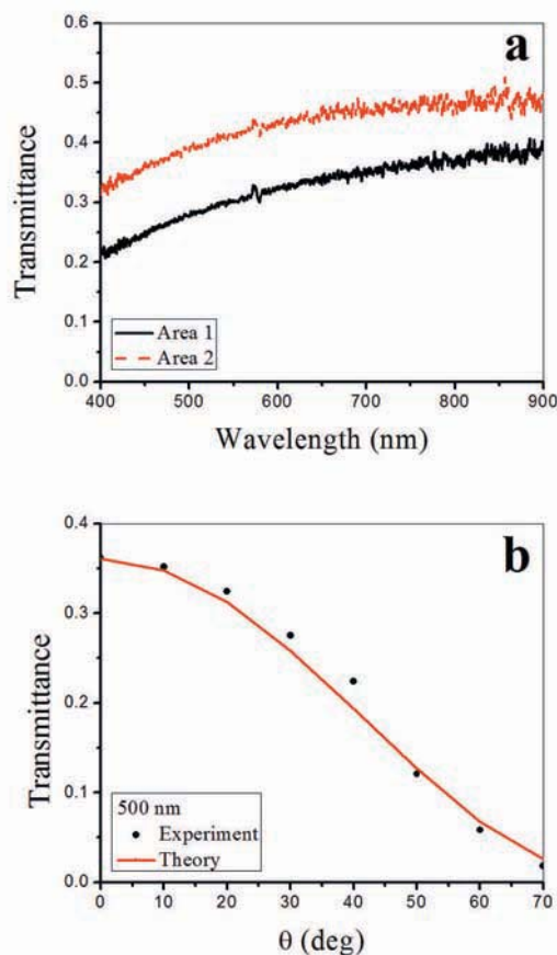
FIG. 9. (a) Measured spectra of the transmittance T_{4}^{\text{unpol}} of the clear transparent areas 1 and 2 for normally incident ( \theta = 0^\circ ) unpolarized light. (b) Circles: measured values of T_{4}^{\text{unpol}} of area 4 for \theta \in [0^\circ, 70^\circ] and \lambda_0 = 500 nm, when the incident light is unpolarized. Solid line: predicted values of (T_s + T_b)/2 of a 550-nm-thick layer of chitin for \theta \in [0^\circ, 70^\circ] and \lambda_0 = 500 nm.
