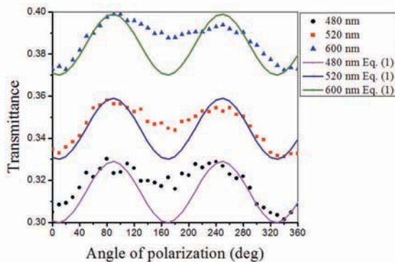
FIG. 10. Transmittance T_{po} of area 1 measured as a function of the angle of polarization \theta_p for normally incident linearly polarized light.
