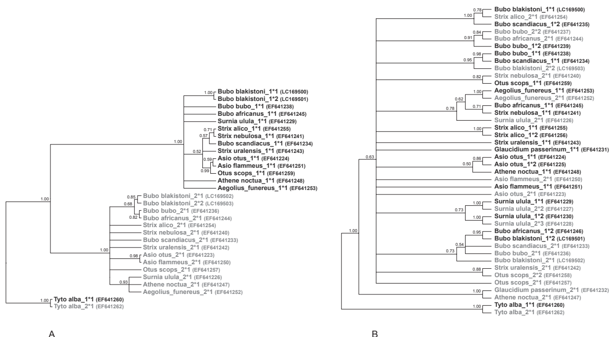
Fig. 1. Phylogenetic relationships among MHC class II \beta exon 3 (A) and MHC class II \beta exon 2 (B) alleles from owl species, reconstructed by Bayesian analysis. Black font, DAB1 alleles; gray font, DAB2 alleles. Numbers near nodes are posterior probability values. Accession numbers for allele sequences are in parentheses.
