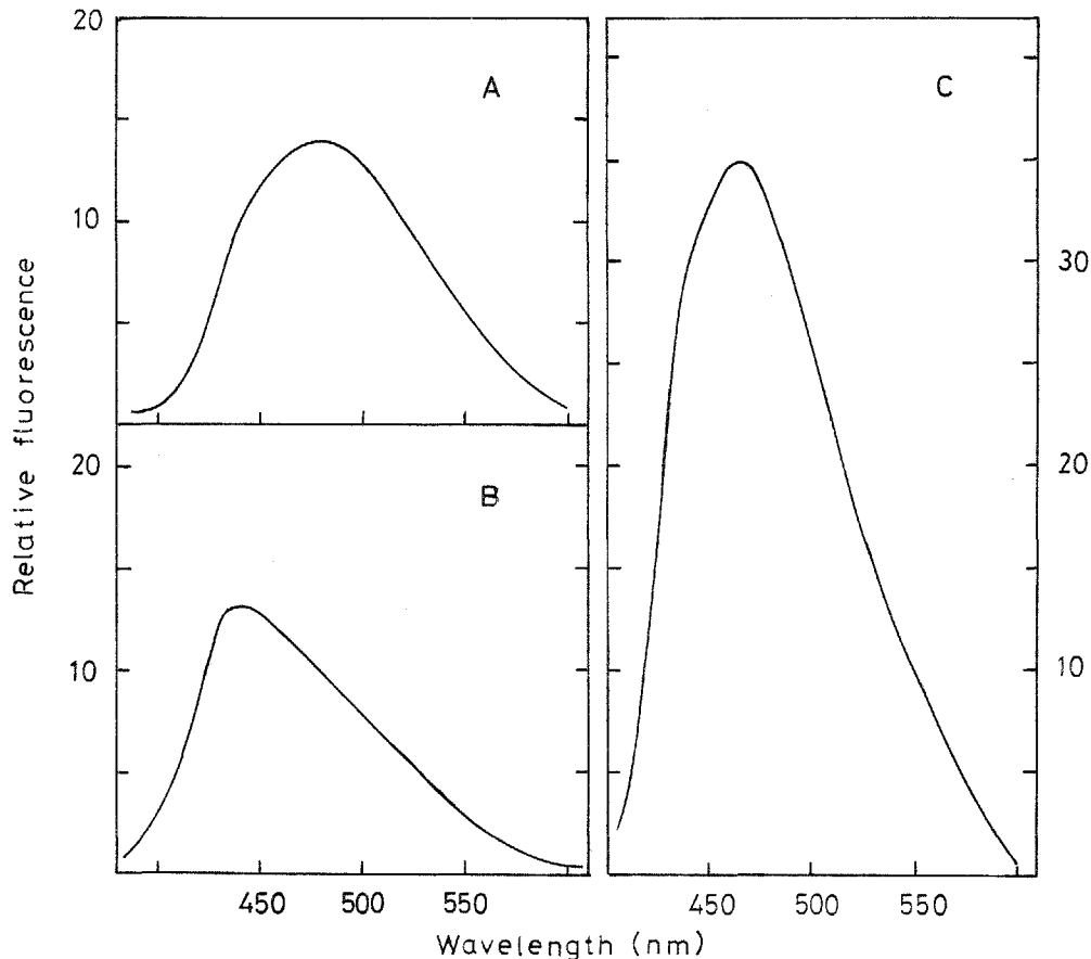
Fig. 2. Fluorescence spectra of granules in Malpighian tubules in early 3rd instar (84 hr) larvae of wild type Or-R (A) and eye color mutants v;bw (B) and cn bw (C). All fluorescence intensities are means for three to six determinations.
