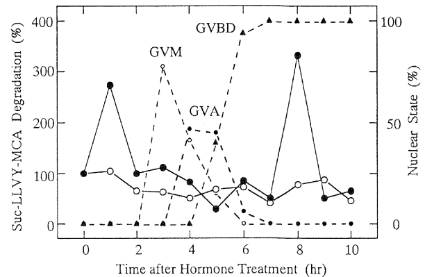
Fig. 1. Changes in the state of the germinal vesicle and the activity of the 26S proteasome during goldfish oocyte maturation. The 26S proteasome activity in the oocyte cytosol from oocytes exposed to 17 \alpha ,20 \beta -DP (●) or ethanol (vehicle of 17 \alpha ,20 \beta -DP) (○), was determined as described in Materials and Methods. The 26S proteasome activity is indicated in arbitrary units with values (%) for activity in the immature oocyte cytosol set at 100%. The status of germinal vesicle during the 17 \alpha ,20 \beta -DP-induced oocyte maturation was also examined (---). GVM, migrating germinal vesicle; GVA, attached germinal vesicle; GVBD, germinal vesicle breakdown.
