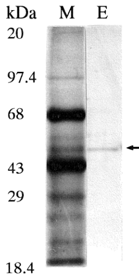
Fig. 5. SDS-PAGE for the purified endo- \beta -1,4-glucanase by silver staining. E, purified endo- \beta -1,4-glucanase (arrow); M, molecular weight standards consisting of myosin H-chain (20 kDa), phosphorylase b (97.4 kDa), bovine serum albumin (68 kDa), ovalbumin (43 kDa), carbonic anhydrase (29 kDa), and \beta -lactoglobulin (18.4 kDa). The molecular weight of the purified endo- \beta -1,4-glucanase was estimated to be 47 kDa.
