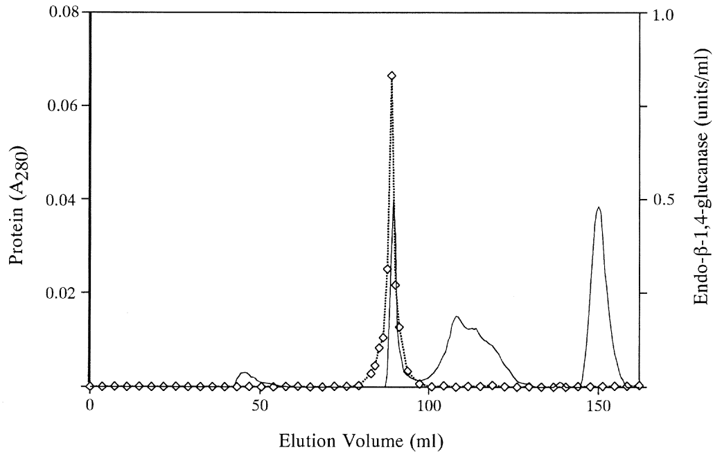
Fig. 6. Elution profile of crude midgut extract on Superdex-75. ( \diamond ) Endo- \beta -1,4-glucanase activity; ( - ) protein measured by absorbance at 280 nm. The endo- \beta -1,4-glucanase activity was eluted in an identical volume ( K_d=0.68 ) to that from whole termites.
