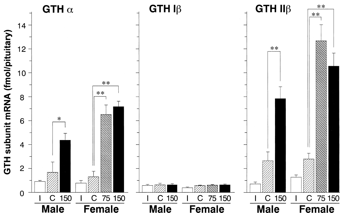
Fig. 1. Changes in the levels of GTH subunit mRNAs in terms of whole pituitary in GnRH \alpha -implanted maturing sockeye salmon. GTH \alpha , I \beta and II \beta subunit mRNA levels in each group are shown. I, initial control; C, control; 75, 75 \mu g of GnRH \alpha -implanted; 150, 150 \mu g of GnRH \alpha -implanted. Mean \pm SEM (n = 3-6). *, P < 0.05 ; **, P < 0.01 ; by the t -test.
