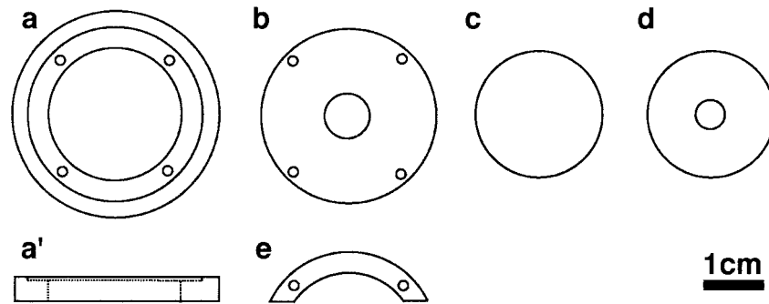
Fig. 2. A sample holder and films used for the observation of blood cells by x-ray microscopy. (a) Stainless steel sample holder. (a') Sample holder viewed from the side. (b) Stainless-steel support with a hole, 8 mm in diameter, at the center. (c) Polyethylene terephthalate (PET) film with a diameter of 22 mm and thickness of 23 \mu\text{m} . (d) Polyimide film with a diameter of 22 mm and thickness of 10 \mu\text{m} . A hole 6 mm in diameter was made at the center of the polyimide film. Freeze-dried blood cells mounted on a copper mesh were attached to a stainless steel support (b) with glue, and fixed to the sample holder (a) with two parts (e) and four screws. Wet living blood cells were placed between two PET films (c) with the polyimide film (d) as a spacer. The three films were attached with silicon grease, placed between two stainless steel supports (b), and fixed to the sample holder (a).
