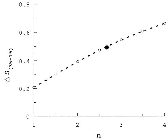
Fig. 7. Influence of cooperativity on the efficiency of O 2 transport by fetal blood at physiological P_{50} . Dotted line represents \Delta S_{(35A-15B)(20)} value calculated from the Hill equation. The closed circle represents the \Delta S_{(35A-15B)(20)} value calculated from the human adult standard OEC.
