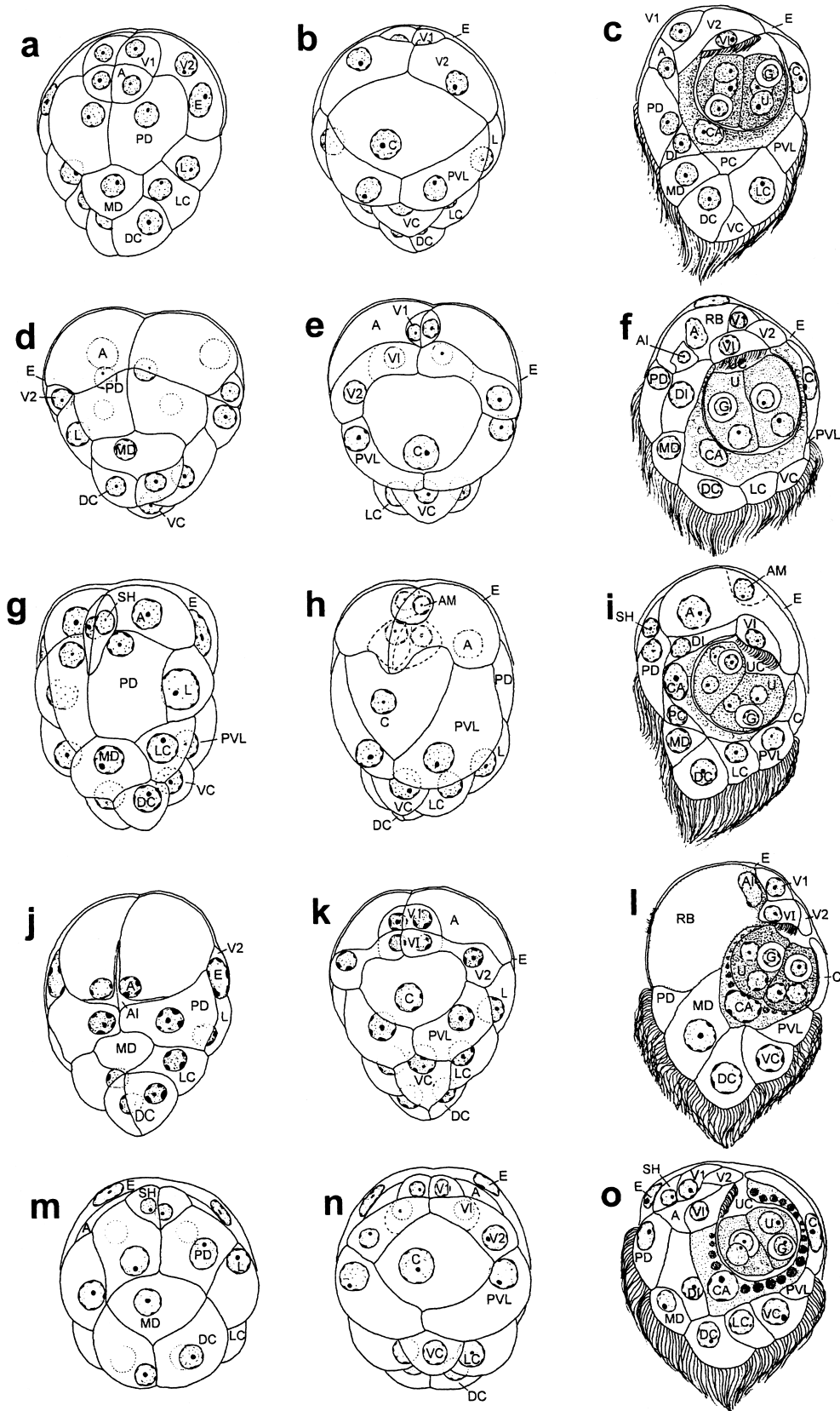
Fig. 6. Sketches of infusoriform larvae. a–c, Dicyema maorum ; d–f, Dicyemenea lameerei ; g–i, Dicyema sp.; j–l, Dicyema acuticephalum ; m–o, Dicyemenea canadensis . a, d, g, j, m (dorsal view); b, e, h, k, n (ventral view); c, f, i, l, o (sagittal section). See Table 1 for abbreviations.
