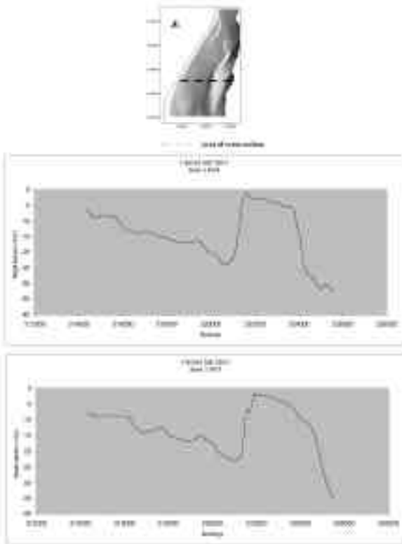
Figure 5. Cross-section profiles from Zone 1 (1844-1873), Co. Wexford.
