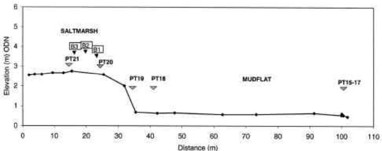
Figure 5. Shore-normal profile at Bridgewick, showing the location of pressure sensors (numbered triangles) and vegetation measurement sites (B1-3)
