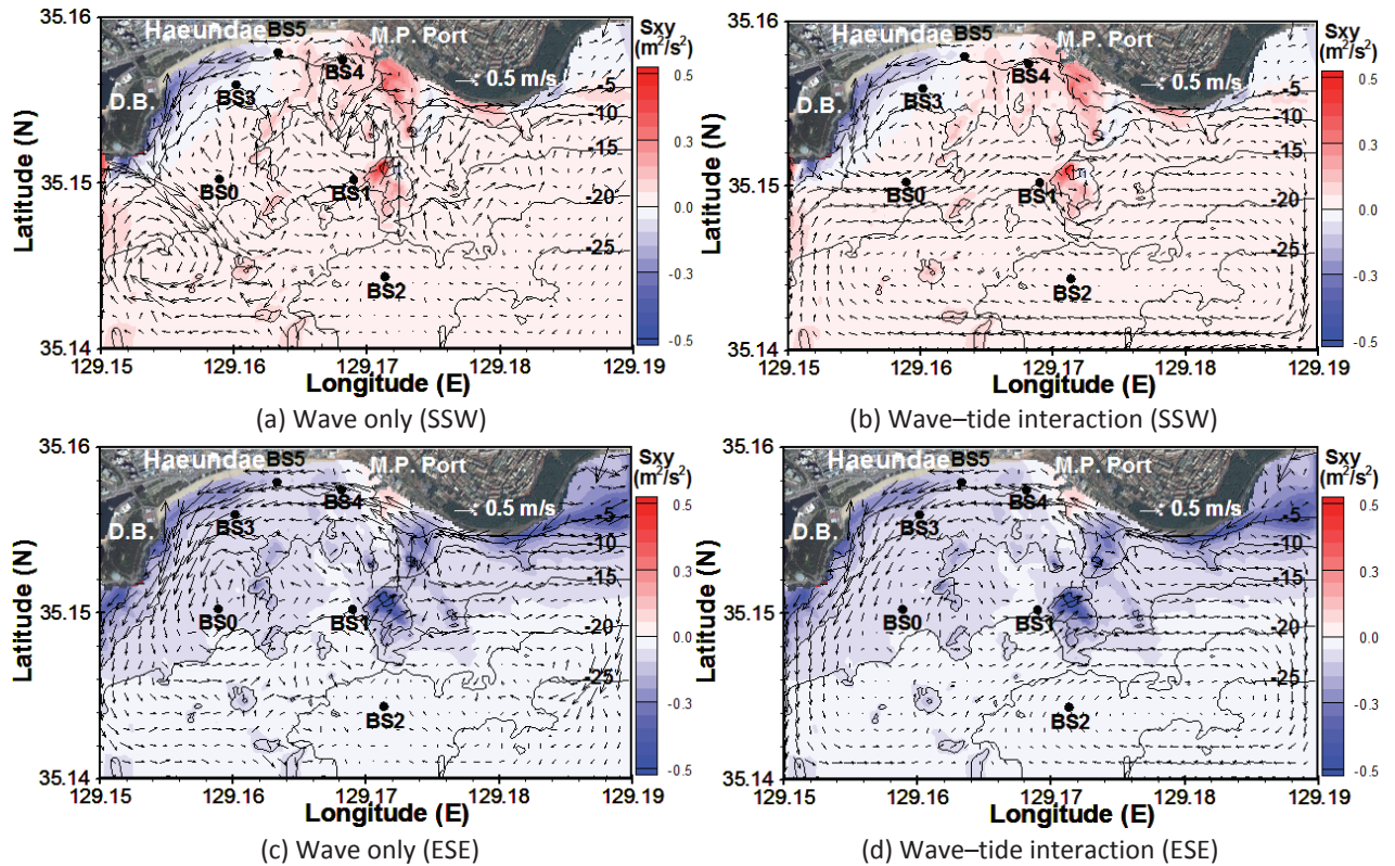
Figure 7. Bottom wave-induced current and horizontal radiation stress ( S_{xy} ) simulated by the ROMS-SWAN model under wave conditions of 2.5 m wave height and 12 s for different wave directions; (a, b) SSW and (c, d) ESE with/without wave–tide interaction.
