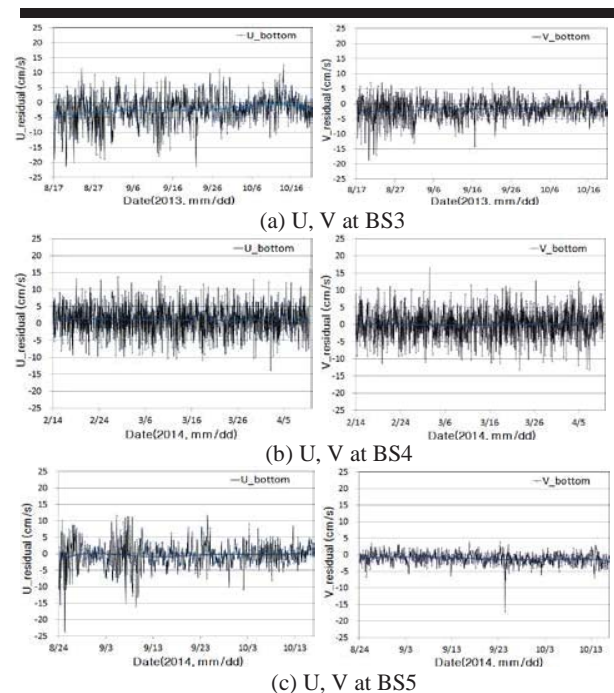
Figure 3. Time series of bottom residual current at (a) BS3, (b) BS4, and (c) BS5 observed nearshore of the beach, derived from measured current data, eliminating predicted tidal current estimated by T_TIDE.
