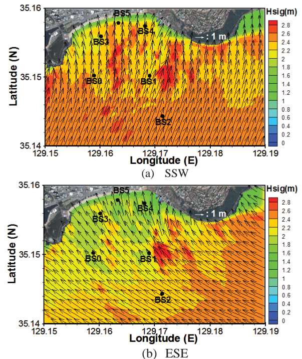
Figure 5. Significant wave height and direction simulated by SWAN model for swell waves ( H_s : 2.5 m, T_p : 12 s) coming from (a) SSW in summer, and (b) ESE in winter.
