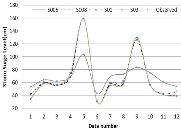
Figure 4. Training Results for Case2 Model Using GRNN.
