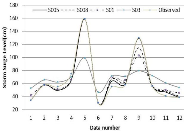
Figure 3. Training Results for Case1 Model Using GRNN.
