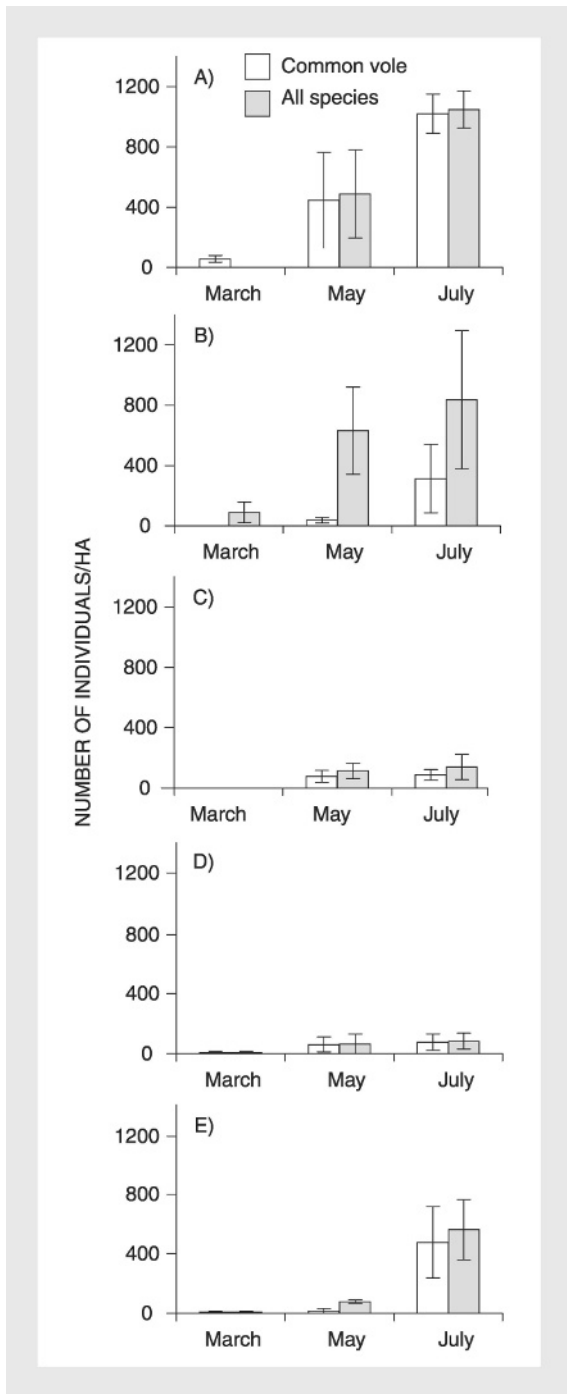
Figure 2. Mean densities of small mammal species ( \pm SE) and mean densities of common voles ( \pm SE), corrected for different capture probabilities, in the five habitat types (A) wild-flower strips, B) herbaceous strips, C) low-intensity meadows, D) artificial grassland and E) autumn-sown wheat) for March, May and July 2003. Capture probabilities: M. arvalis = 0.22, M. agrestis = 0.39, A. sylvaticus = 0.22, A. flavicollis = 0.25, C. glareolus = 0.19.
