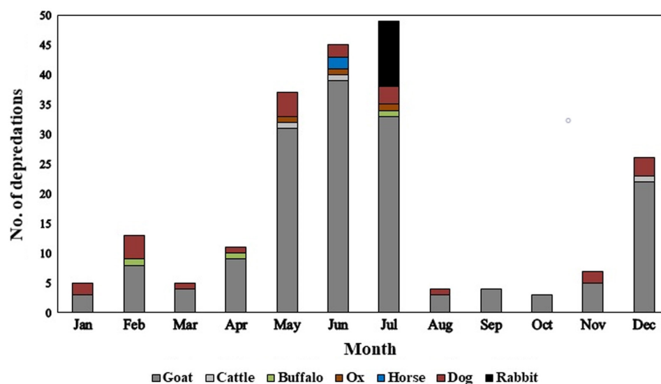
Figure 2. Monthly frequency of common leopard Panthera pardus deprecations on livestock in and near Pir Lasura National Park, Pakistan, 2014–2015.
