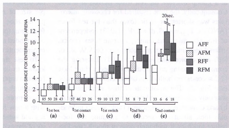
Figure 2. Time (in seconds) from the moment the foxes entered the arena ( t_{in} ) until they a) reached the first food box, b) had the first contact with a lemming or a vole, c) switched to the second food box, d) reached the second food box and e) had the second contact with a lemming or a vole. Note that c), d) and e) were no longer of necessity if the first contact b) was a choice. Vice versa, physical contact was not necessary for refusing and side switching. Cases of foxes ordered to go out of the arena were excluded. Bars indicate medians, first and third quartiles and ranges.
