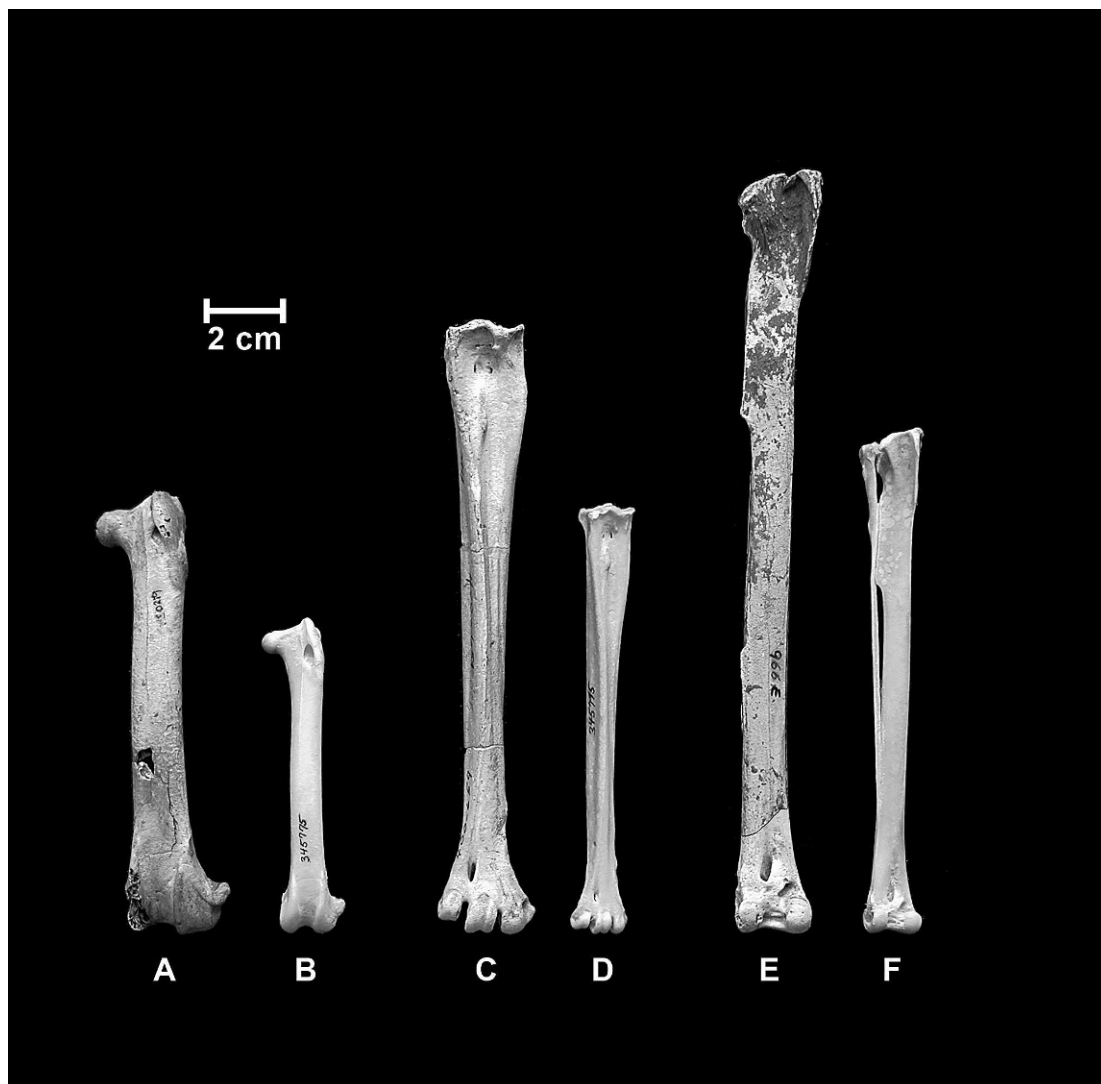
Figure 3. Hindlimb elements in anterior view of Buteogallus borrsi (A, C, E) compared with B. urubitinga (USNM 345775; B, D, F). A, left femur (WS 1115); C, right tarsometatarsus (CZACC 400-659); composite right tibiotarsus (proximal WS 966E, distal WS 971).
