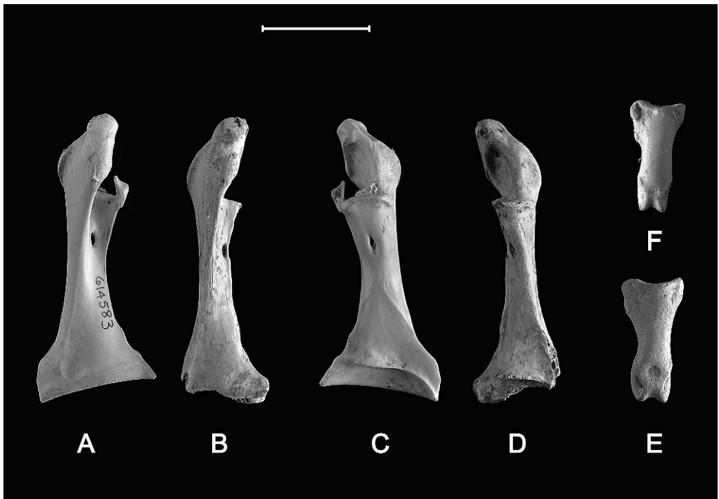
Figure 5. Right coracoids (A, B, ventral view; C, D, dorsal view) and pedal phalanx I of digit I in dorsal view (E, F) of Caracara . A, C, F, C. plancus USNM 490931; B, D, C. telluris , new species, USNM 535725; E, C. tellustris , new species, USNM 535729. Scale = 2 cm.
