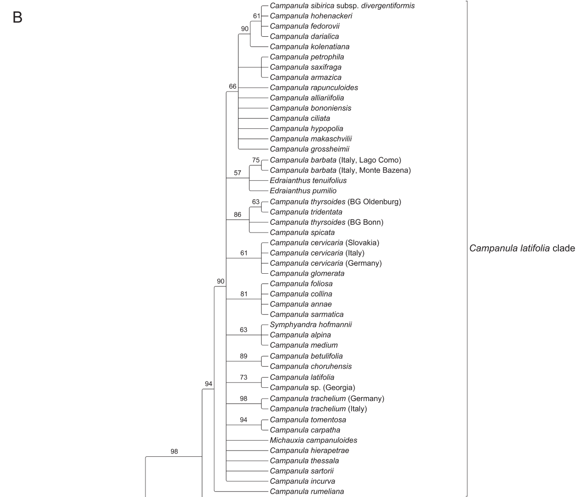
Fig. 4A-B. Maximum Parsimony tree of Campanulaceae (strict consensus of 229 shortest trees of 1525 steps) based on the petD data set including indels. – Jackknife values supporting individual nodes are shown above branches.
