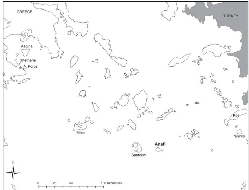
Fig. 1. The South Aegean Volcanic Arc.
