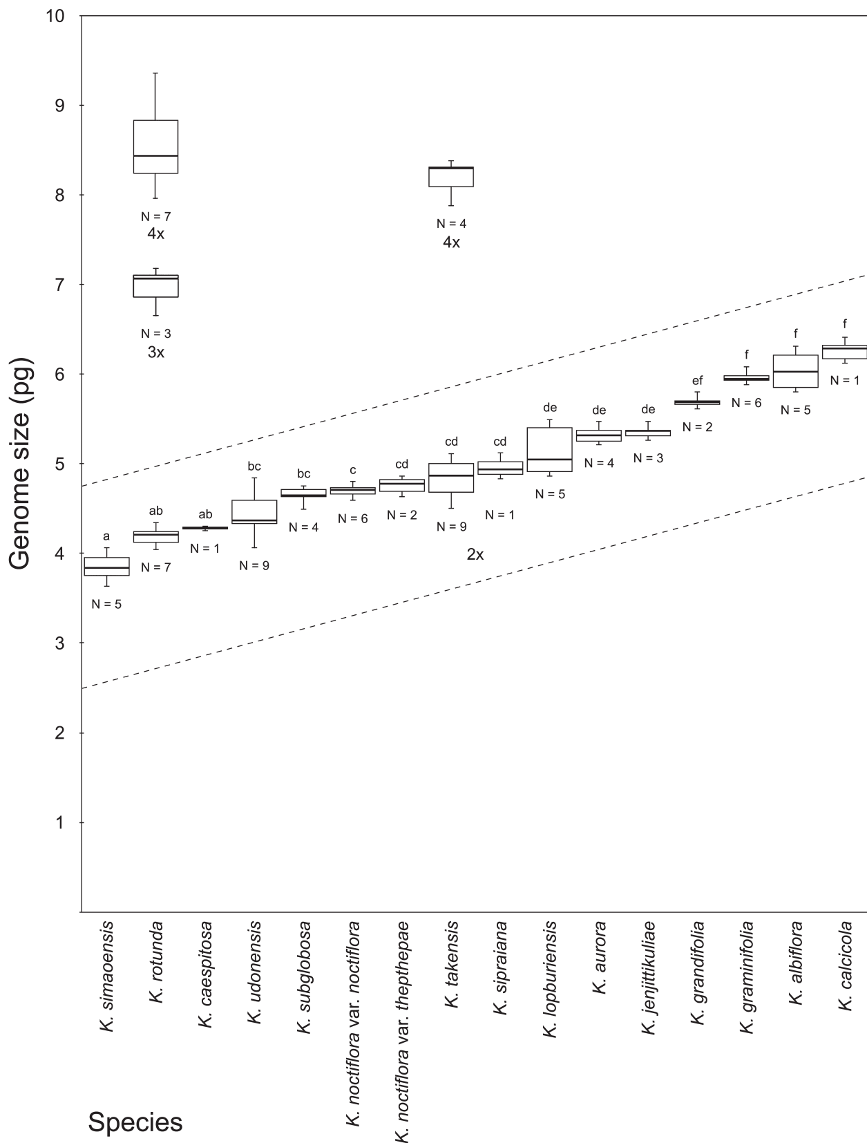
Fig. 4. Boxplot representing range of genome sizes (in picograms) of species of Kaempferia subg. Protanthium in Thailand based on 84 accessions (276 individual plants) from 15 species and one variety. Lines extending from boxes (whiskers) indicate variability outside upper and lower quartiles. Different letters above each box indicate statistically significant difference between means of genome sizes ( p < 0.05 ). – N = number of accessions included in flow cytometry analysis. – 2x = diploid; 3x = triploid; 4x = tetraploid. Mean genome size with standard deviation data of individual plants follows Appendix S2.
