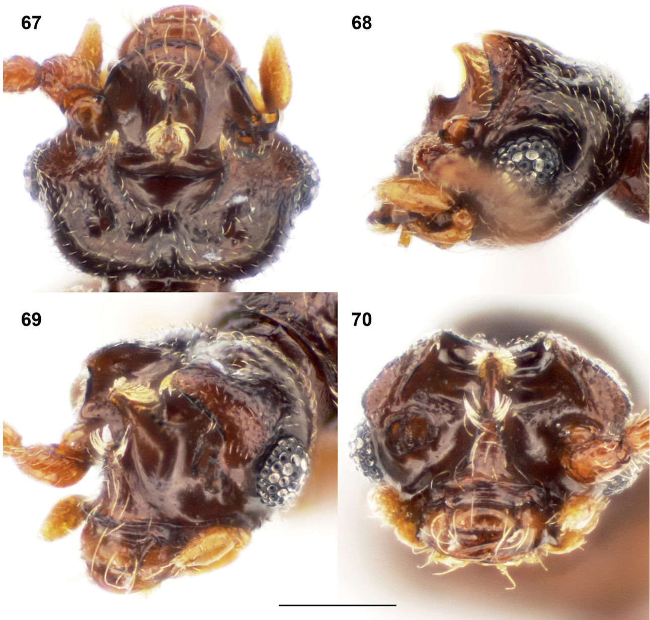
Figs 67-70. Achilia elguetai n. sp. Male head in (67) dorsal, (68) lateral, (69) semilateral, and (70) frontal views. Scale bar (200 \mu m).
