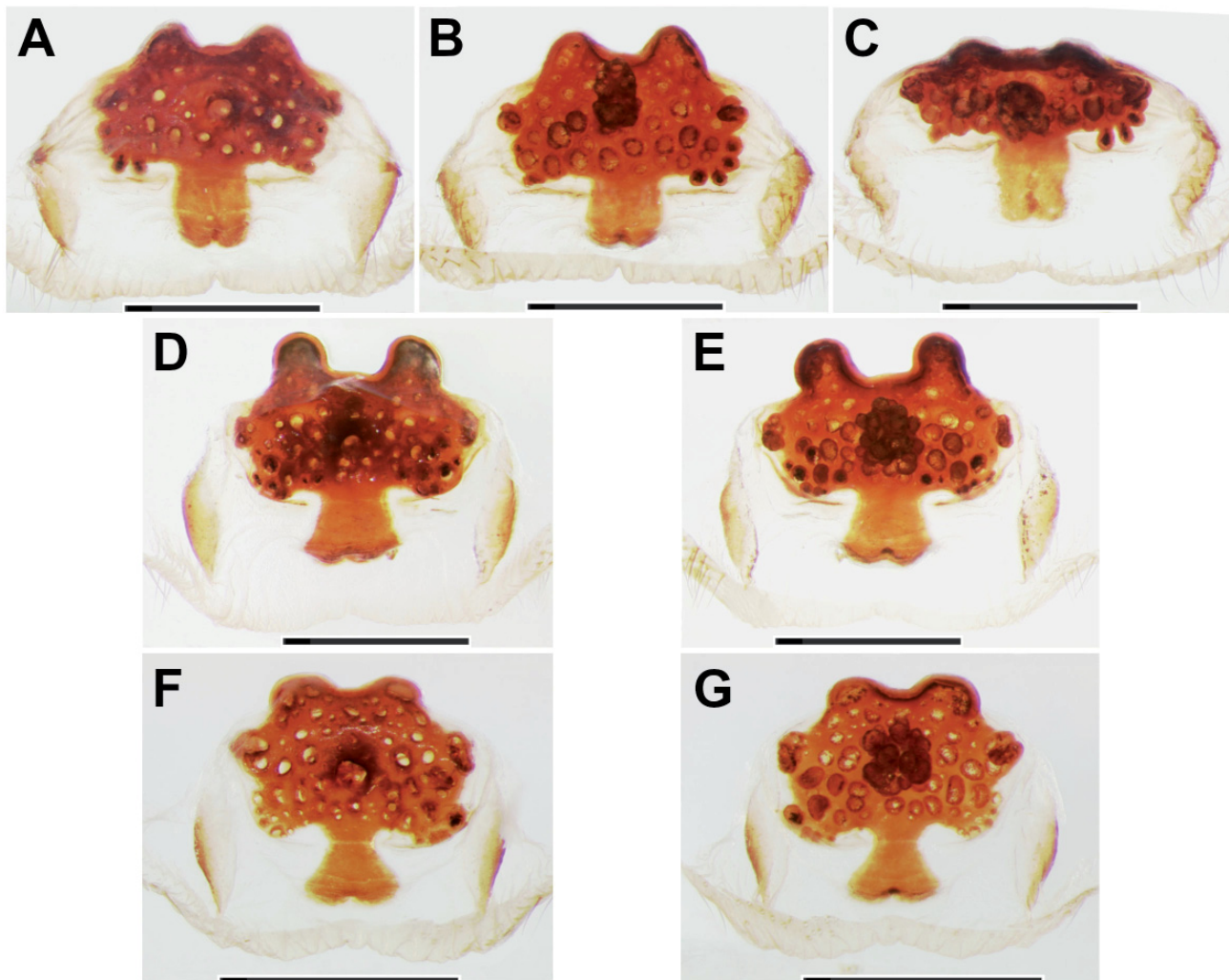
Fig. 20. Liphistius pyinoolwin , vulval plates of three females (all taken from exuviae), dorsal view (A, D, F), ventral view (B, E, G) and ventral and slightly anterior view (C). (A-C) Moults of 1.IX.2017. (D-E) Moults of 15.X.2017. (F-G) Moults of 22.I.2016. Scale lines 1.0 mm.
