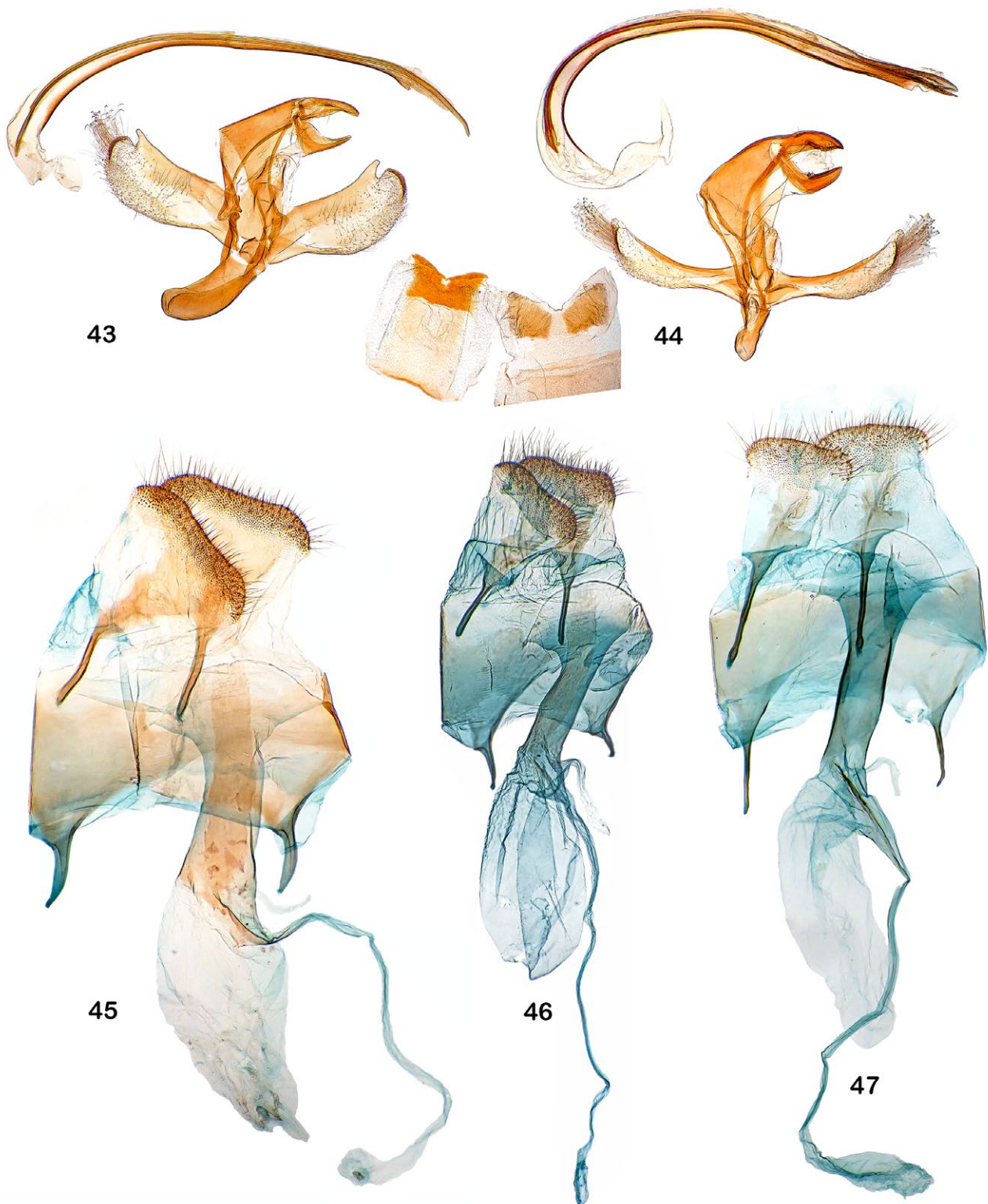
Figs 43-47. Ancyolomia spp., male and female genitalia. (43) A. savutiensis sp. nov., male holotype. (44) A. medioafricana sp. nov., male holotype and sclerites of abdominal segment VIII. (45) A. lucia sp. nov., female holotype. (46) A. trematerrai sp. nov., female holotype. (47) A. lydia sp. nov., female paratype.
