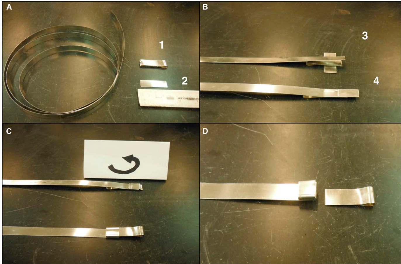
Fig. 1. Constructing a collar on a dendrometer band using the traditional method (from Cattellino et al., 1986). (A) Cut a short section (5–8 cm) from the banding material and fold it back into a loop to create a spacer tool (1), to be reused for making the collar on each dendrometer band. For the collar, cut a section of banding material about three times longer than wide (2); set it aside for the next step. To estimate the length of dendrometer band to cut, measure the tree circumference where the band will be placed (at breast height) and add 20–30 cm to the length of banding material. (B) At one end of the dendrometer band, form the collar by placing the spacer loop under the band as shown (3), with the short piece of banding material held under both the spacer and band, near the end at about the same distance as the width of the band. Fold both sides of the short piece of band up around the spacer tool and the end of the band, forming the collar (4). (C) Fold the end of the band back over the collar, and using the spacer tool for leverage, fold the end of the band again so that the collar ends are concealed and the collar is locked at the end of the band. (D) Pull the spacer tool free of the collar; there should be a gap large enough for the free end of the dendrometer band to be inserted into the collar and move easily as the tree grows. The band and collar are now ready for installation.
