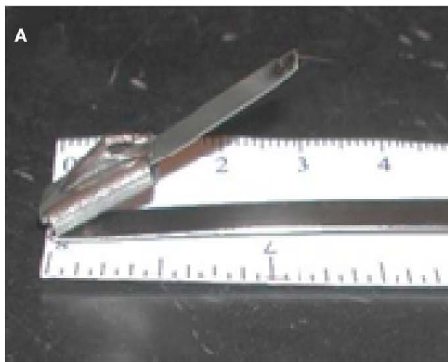
Fig. A2. Attaching the dendrometer band collar. (A) Slip a collar on the short section with the “tab” end of the collar away from the bend. (B) Fold the protruding short end of band under the collar and crimp the folds to secure the collar.
