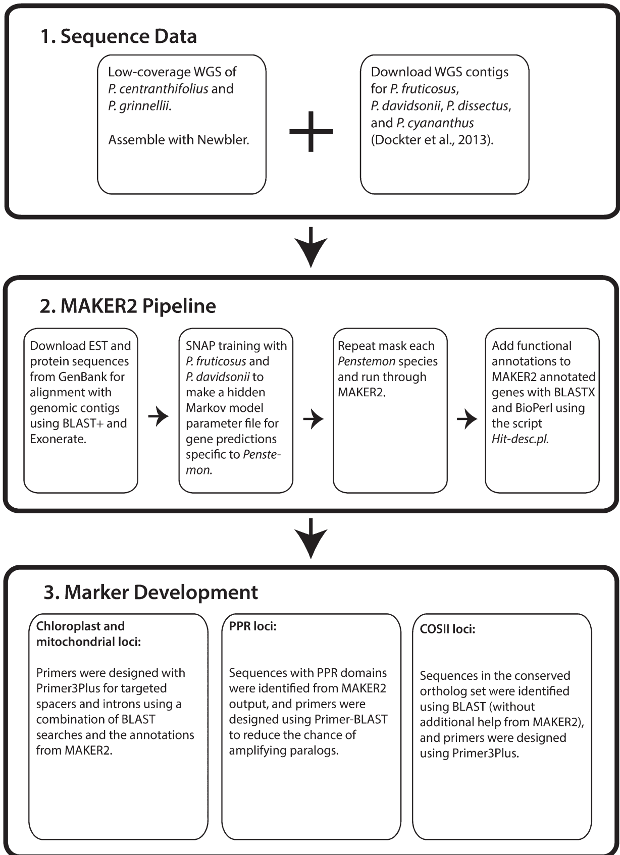
Fig. 1. Workflow used for marker development from six low-coverage Penstemon genomes using the MAKER2 Annotation Pipeline.
