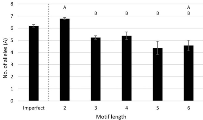
Fig. 2. Comparison of the number of alleles across different motif lengths. There are significant differences in the motif lengths overall according to the Kruskal–Wallis test; letters above each category depict significantly different groupings based on DSCF posthoc comparisons to further characterize these differences. These groupings indicate that the dinucleotide repeats (2) are significantly different from most other motif lengths. Imperfect motifs are included for side-by-side comparison but were not included in statistical analysis. Error bars represent the standard error of each mean.
