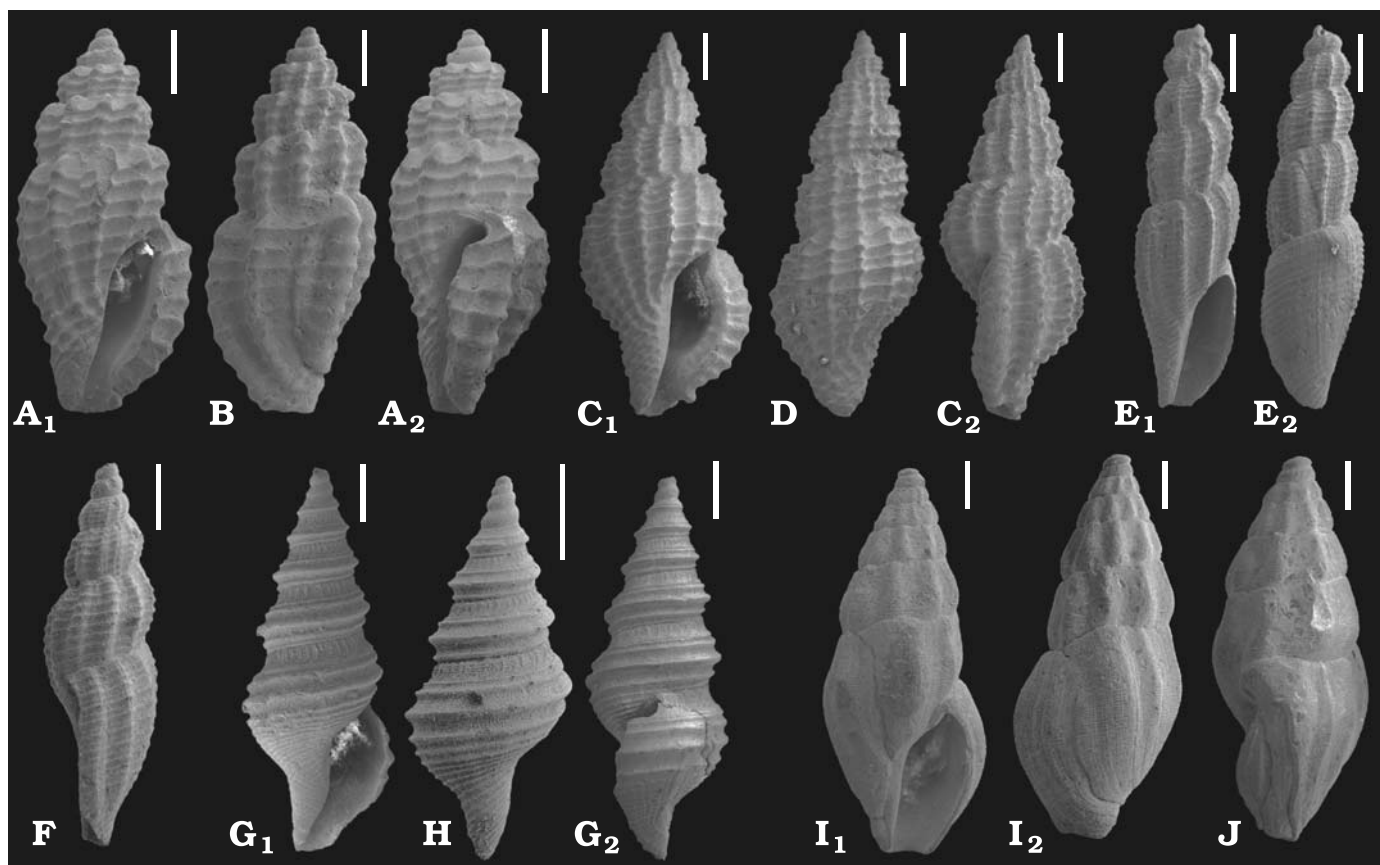
Fig. 8. SEM images of shell features of conoidean gastropods from early Serravallian of western Ukraine, Horodok (A, B) and Varovtsi (C–J). A, B. Pyrgocythara turrspiralata sp. nov. A. MGGC-24515/11. B. MGGC-24515/9. C, D. Raphitoma cf. R. ringicula (Boettger, 1902). C. MGGC-24522/1. D. MGGC-24522/3. E, F. Andonia sp. aff. A. transsilvanica (Hoernes and Auinger, 1890). E. MGGC-24523/1. F. MGGC-24523/3. G, H. Teretia cf. T. turriloides (Bellardi, 1847). G. MGGC-24524/3. H. MGGC-24524/5. I, J. Haedropleura sp. aff. H. septangularis (Montagu, 1803). I. MGGC-24520/6. J. MGGC-24520/11. Views: A 1 , C 1 , E 1 , G 1 , I 1 , apertural; B, D, E 2 , H, I 2 , dorsal; A 2 , C 2 , F, G 2 , J, lateral. Scale bars 1 mm.
