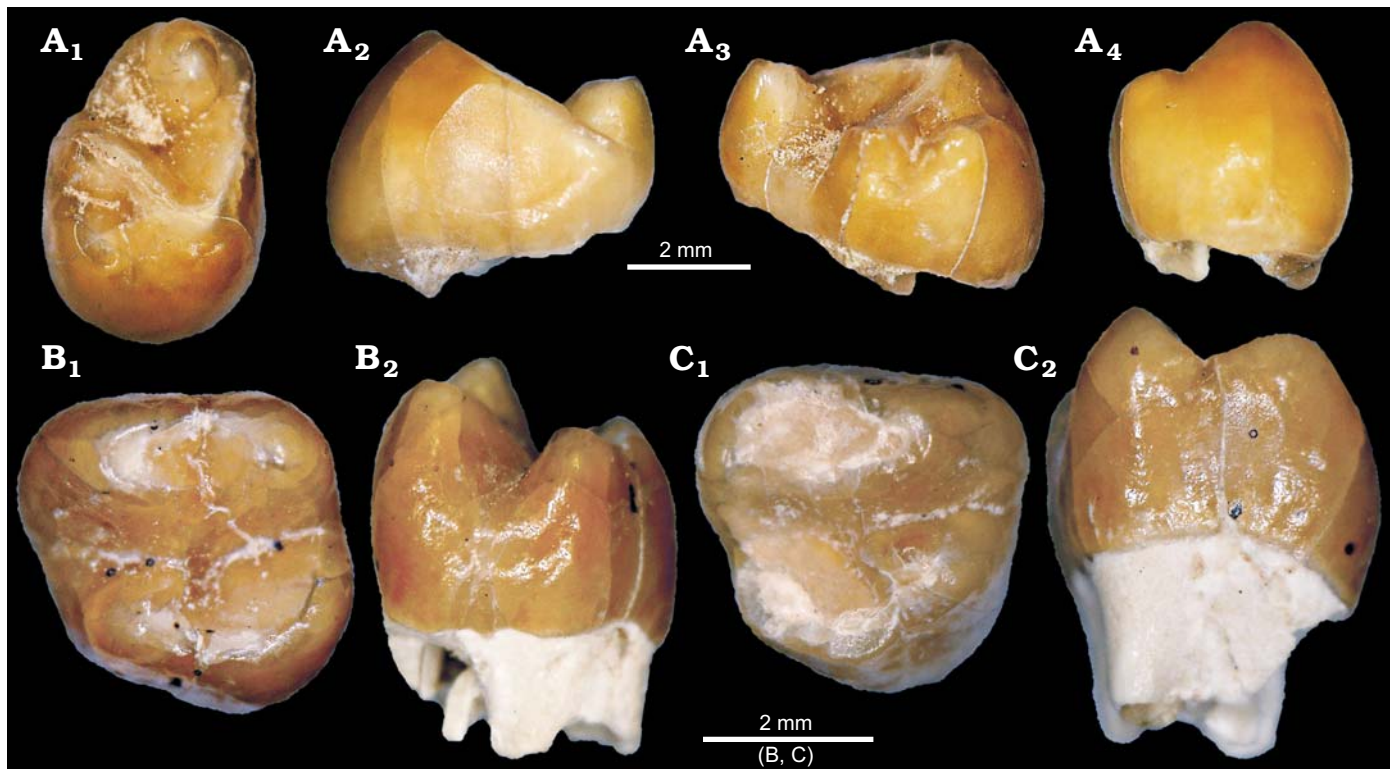
Fig. 3. Mimotonid Gomphos progressus sp. nov. from the Eocene of Wulanhuxiu, Nei Mongol, China. A. Left M3 (IVPP V20824) in occlusal (A 1 ), anterior (A 2 ), posterior (A 3 ), and lingual (A 4 ) views. B. Left m2, holotype (IVPP V20259) in occlusal (B 1 ) and buccal (B 2 ) views. C. Right m3 (IVPP V20259.1) in occlusal (C 1 ) and anterior (C 2 ) views.
