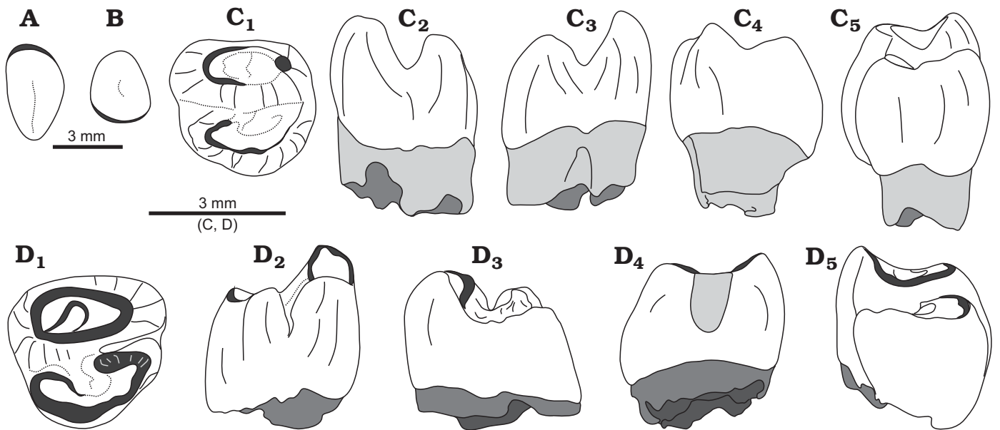
Fig. 4. Morphology of tooth of Gomphos progressus sp. nov. A. Cross-section of the left upper incisor (IVPP V20259.2). B. Cross-section of the left lower incisor (IVPP V20259.3). C. Left m2, holotype (IVPP V20259) in occlusal (C 1 ), buccal (C 2 ), lingual (C 3 ), anterior (C 4 ), and posterior (C 5 ) views. D. Right m3 (IVPP V20259.1) in occlusal (D 1 ), buccal (D 2 ), lingual (D 3 ), anterior (D 4 ), and posterior (D 5 ) views.
