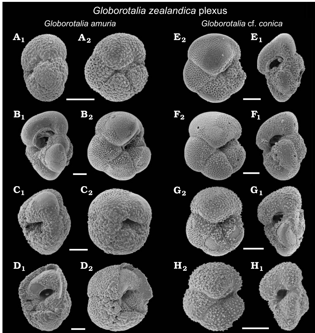
Fig. 4. Middle Miocene planktonic foraminifer Globorotalia zealandica plexus from ODP Site 747, Kerguelen Plateau. A–D. Globorotalia amuria . Encrusted: 8H-1, 38–40 cm (A); 8H-6, 28–30 cm (C); 9H-3, 98–100 cm (D). Non-encrusted: 8H-3, 100–102 cm (B). E–H. Globorotalia cf. conica . Non-pustulose: 8H-2, 128–130 cm (E); 8H-6, 146.5–148.5 cm (F). Pustulose: 9H-1, 4–6 cm (G); 9H-4, 148–150 cm (H). A 1 –H 1 axial view, A 2 –H 2 umbilical view. All SEM images. Scale bars 100 \mu m. The stratigraphic position of pictured specimens is indicated on Fig. 3.
